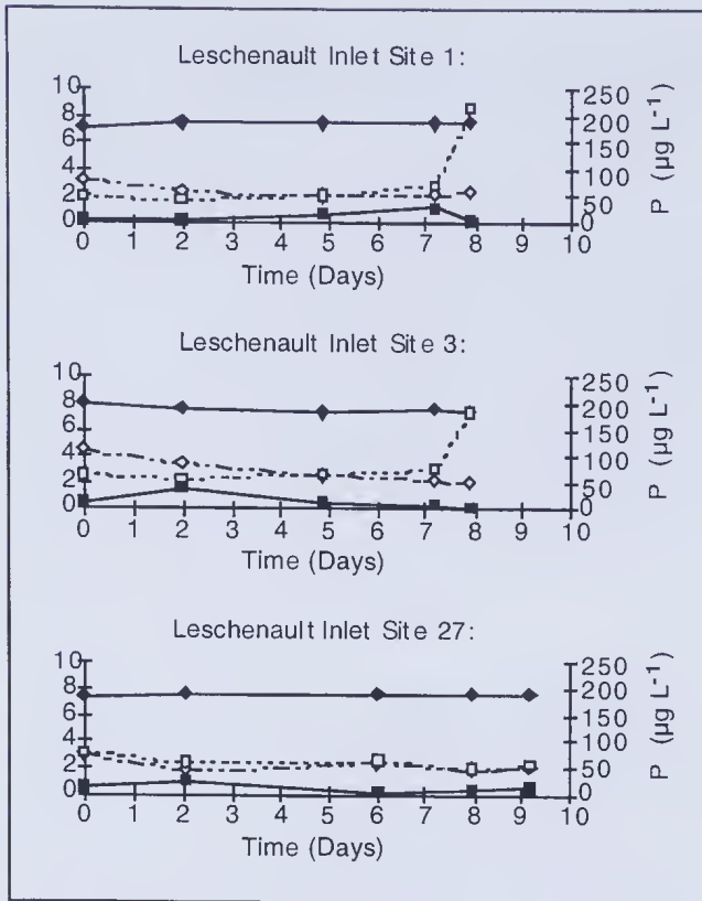
Figure 5. Phosphorus (SRP and TP) release and related pH and DO concentrations (mg L -1 ) in intact cores collected in March 1990 from Leschenault Inlet. Site 1; Site 3; Site 27. —◆— pH; - -◆- - - DO; —■— SRP; - -□- - - TP.
